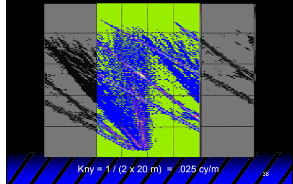
Trace Interval = 20 m F-K Domain
