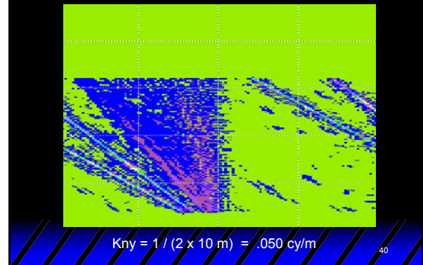
Trace Interval = 10 m by F-X Prediction Filtering F-K Domain
